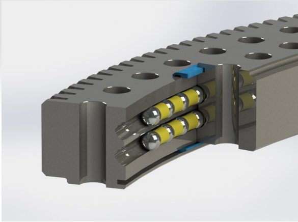
Eight point contact
