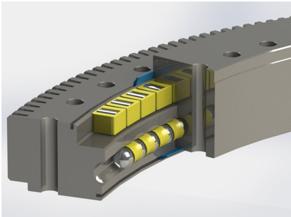
Ball roller combination
