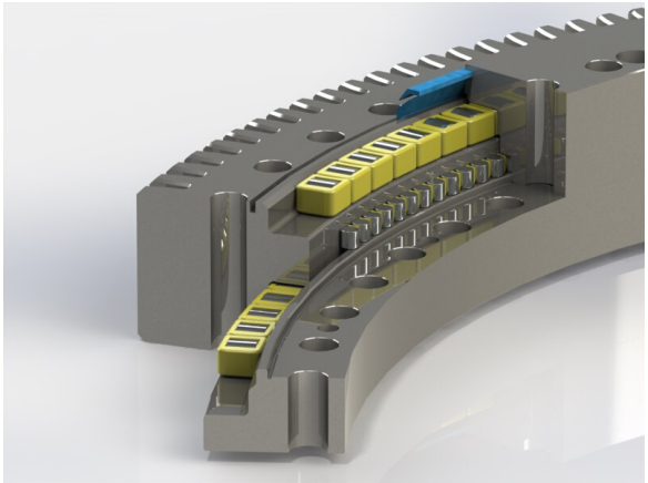
Three row roller
