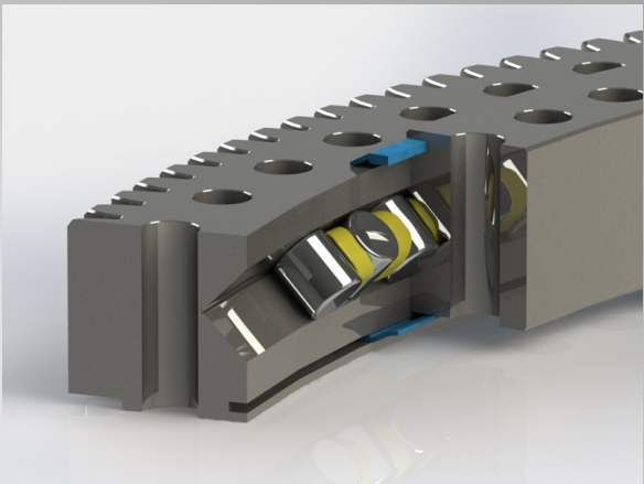
Single row cross roller
