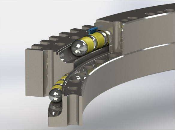
Eight point contact split ring
