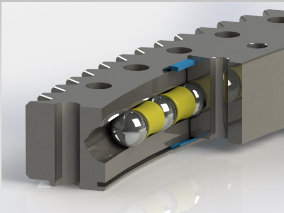
Four point contact
